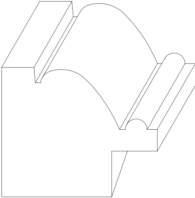
W-237 2 1/8" x 2 9/16" * 3/4" x 3/4" RABBET
