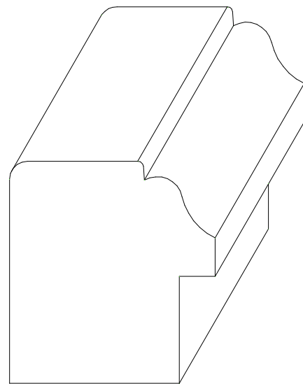
W-1449 1 9/16" x 1 7/16" * 1/4" x 3/4" RABBET
