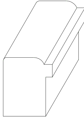
W-78B 1 1/8" x 15/16" * 1/8" x 3/4" RABBET
