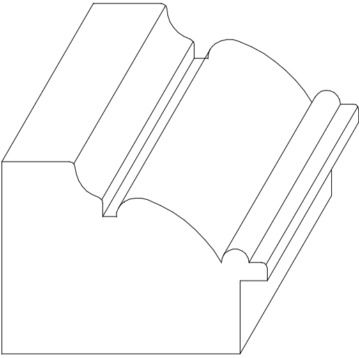
W-2283A 1-5/16" x 1-13/16" * 3/16" x 1/2" RABBET
