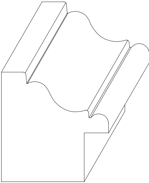
W-2077 1 11/16" x 1 11/16" * 3/8" x 3/4" RABBET
