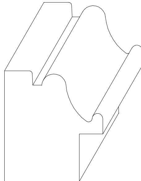
W-1090 1 3/4" x 1 9/16" * 3/8" x 3/4" RABBET
