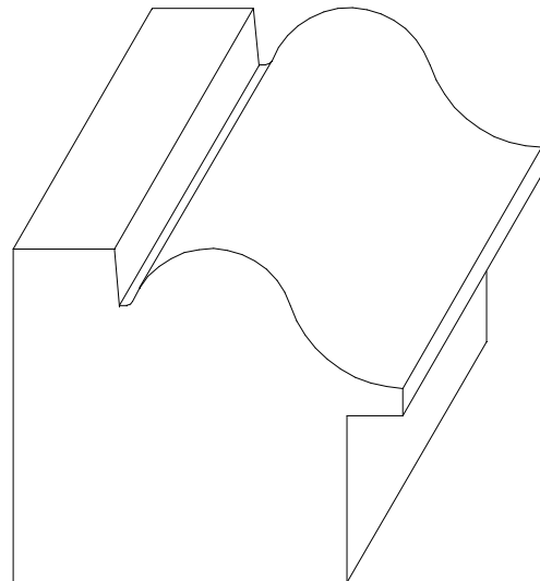
W-1379 1 1/2" x 1 3/4" * 1/4" x 3/4" RABBET
