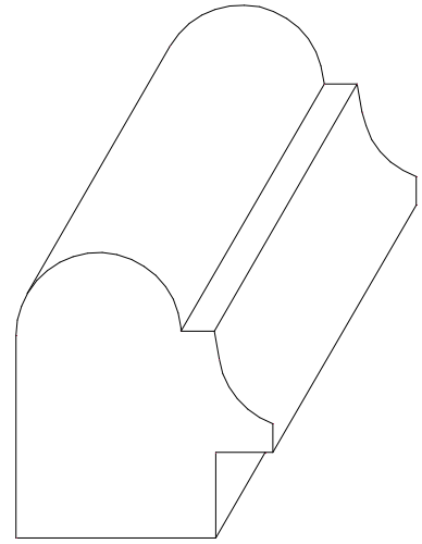
W-2492 1-1/4" x 1-1/8" * 1/4" x 3/8" RABBET
