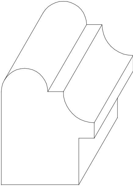
W-1465 1 1/2" x 1 7/8" * 1/4" x 3/4" RABBET
