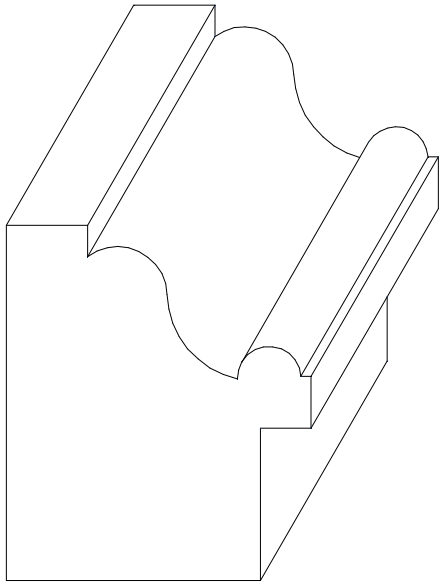
W-336 1 3/4" x 1 1/2" * 1/4" x 3/4" RABBET
