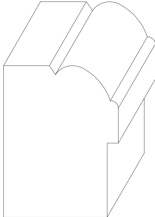
W-2003 2 9/16" x 1 15/16" * 3/16" x 1 1/4" RABBET
