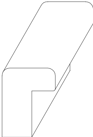
W-1326 1 1/8" x 7/8" * 3/8" x 3/4" RABBET
