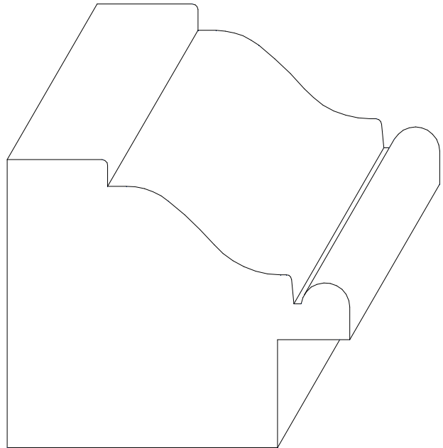
W-793 2" x 2 3/8" * 1/2" x 3/4" RABBET
