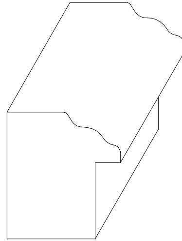
W-1850 1 1/4" x 1 1/8" * 1/4" x 3/4" RABBET
