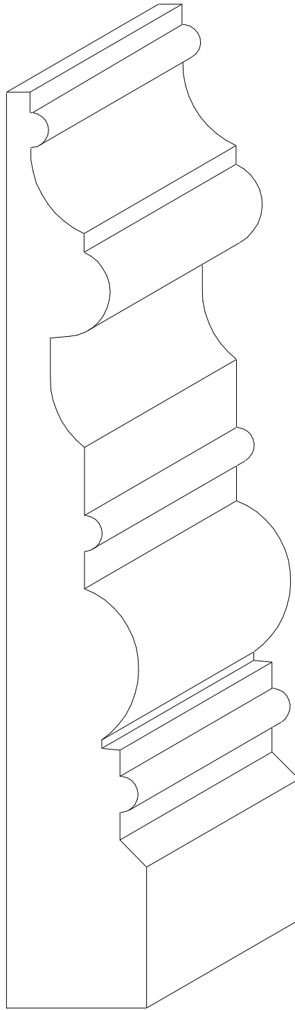
W-457 1" x 6 1/2"
