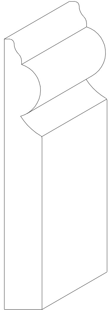
W-294 5/8" x 4 1/2"
