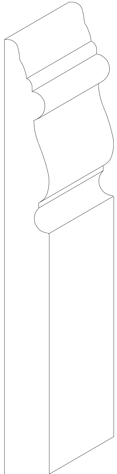
W-248 3/4" x 7 1/4"
