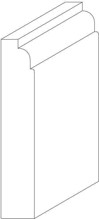
W-589 9/16" x 3"
