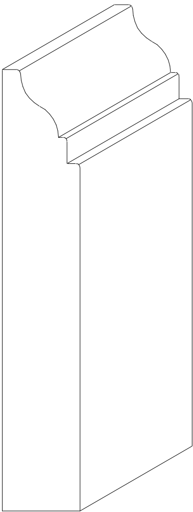
W-471 3/4" x 4 1/4"
