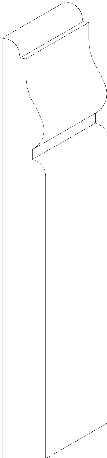
W-409 3/4" x 7 1/4"
