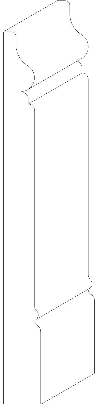
W-112 3/4" x 7 1/2"
