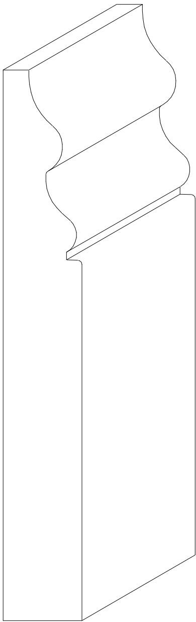
W-306 3/4" x 5-1/4"
