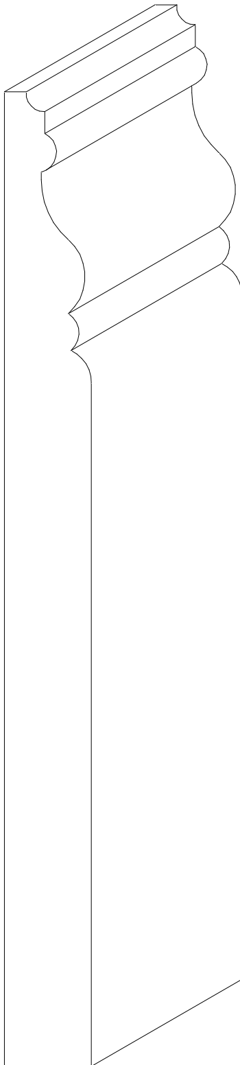
W-540 5/8" x 7"
