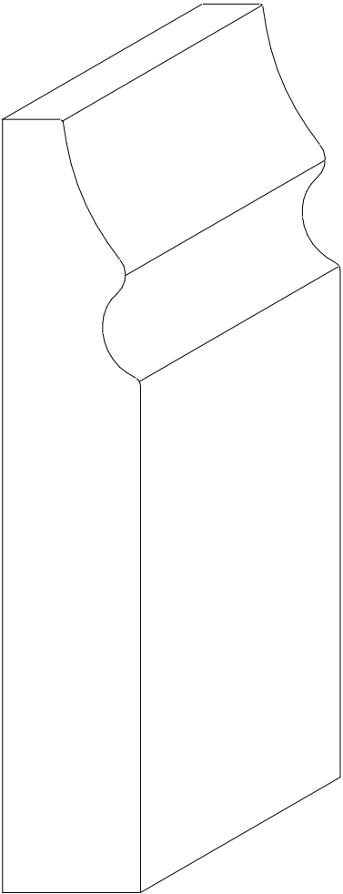
W-104 3/4" x 4 3/16"
