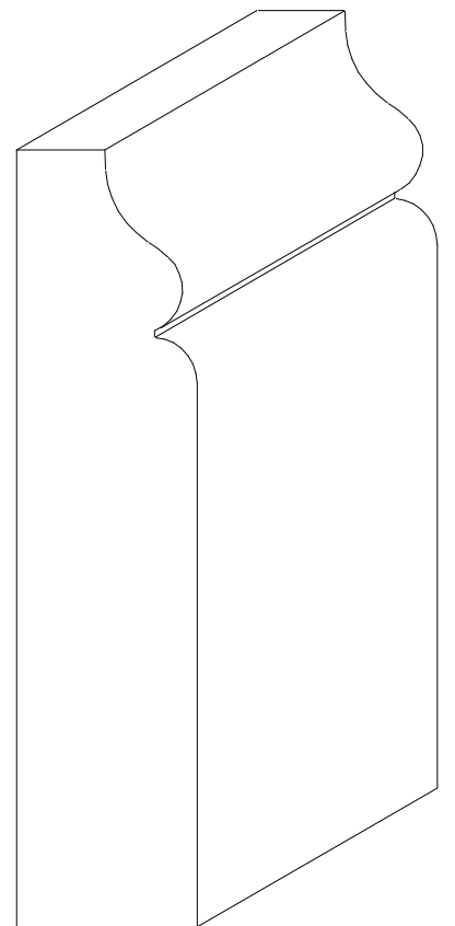
W-484 13/16" x 3 1/2"
