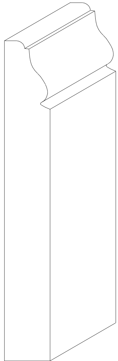
W-184 3/4" x 5 1/4"
