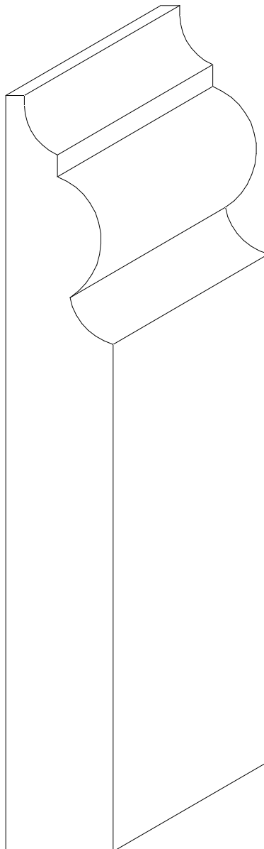
W-438 3/4" x 5 1/4"
