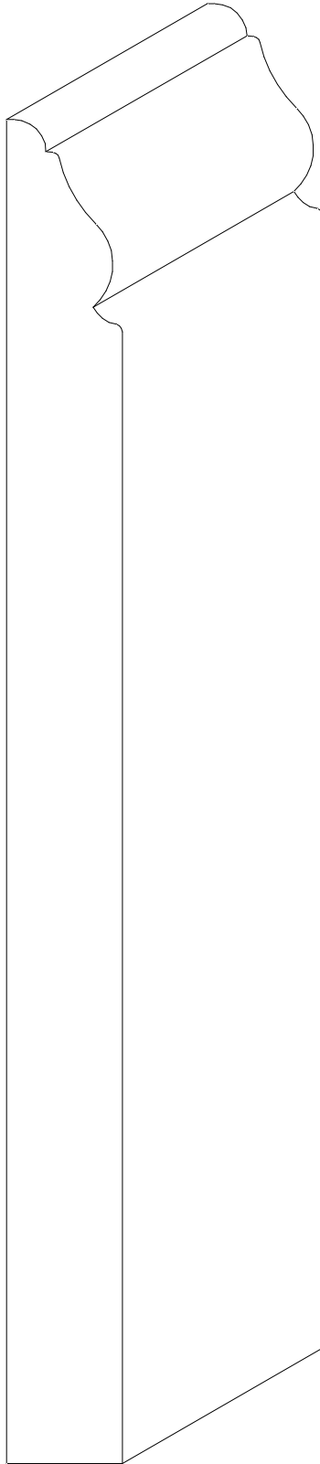
W-110 5/8" x 7 1/4"
