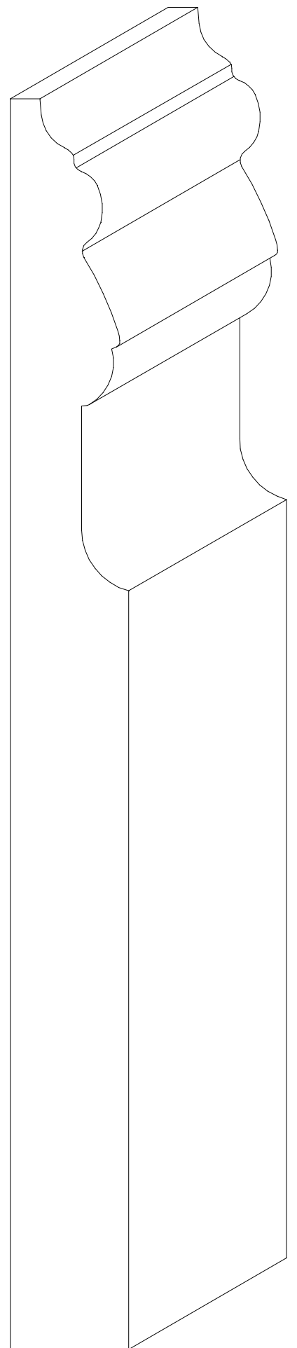
W-2366 13/16" x 8-1/2"
