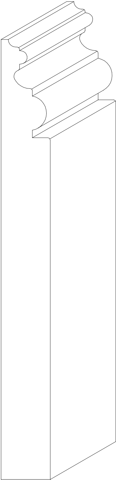
W-2280 13/16" x 7-1/4"
