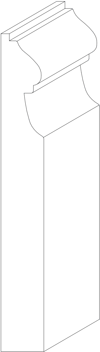
W-2471 13/16" x 6-1/8"
