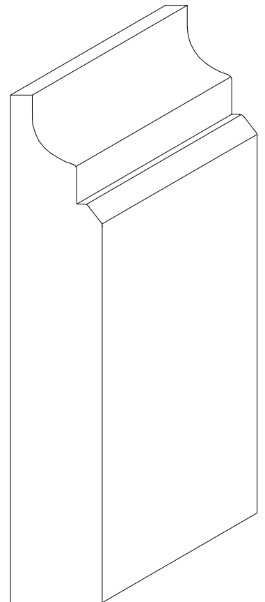
W-2302 5/8" x 3-1/2"
