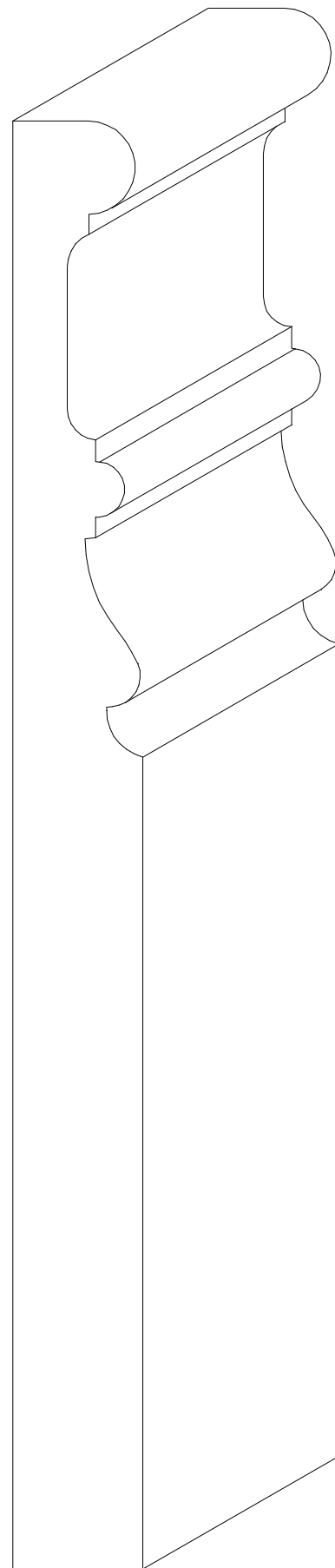
W-2422 3/4" x 8"
