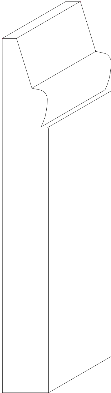
W-2543 3/4" x 6"
