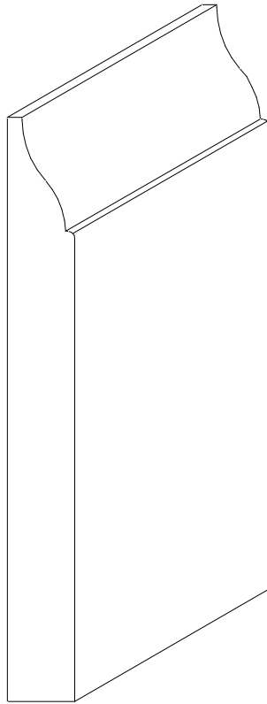
LWM634 3/8" x 3 1/4"
