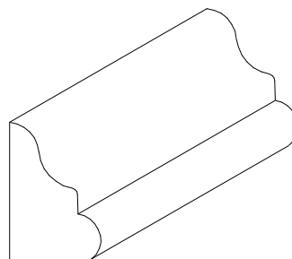
W-1335 .780" x 1/2"
