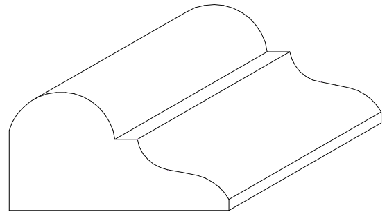
W-675 27/32" x 1 9/16"
