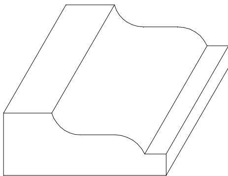
W-938 5/8" x 1 5/8"
