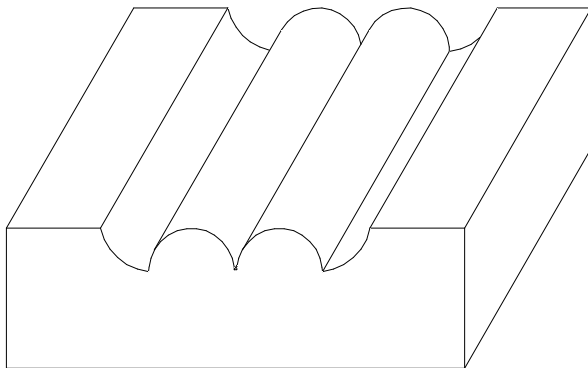
W-918 11/16" x 2 1/4"
