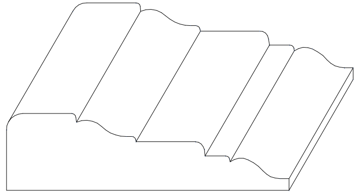
W-1144 3/4" x 2 3/4"
