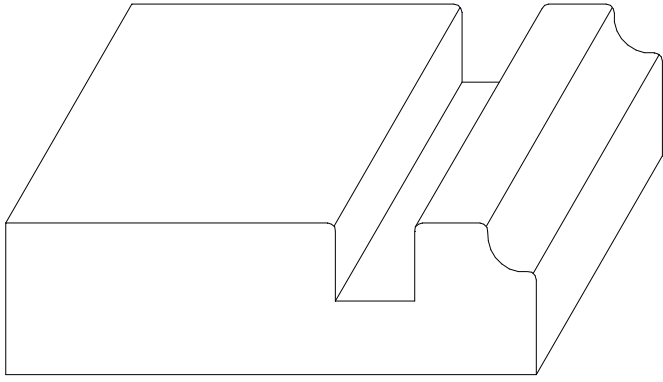
W-1103 3/4" x 2 5/8"
