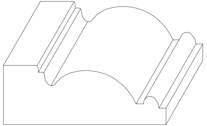
W-1976 1" x 2 3/4"
