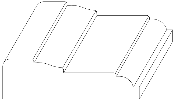
W-1682 3/4" x 2 9/16"
