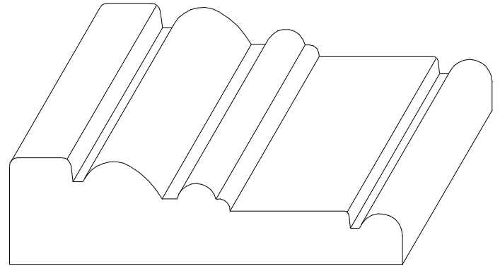
W-259 3/4" x 2 3/4"
