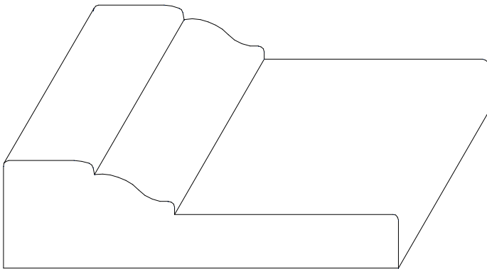
W-1188 3/4" x 2 3/4"
