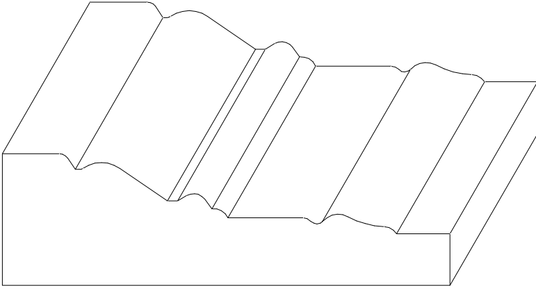
W-26 15/16" x 3 3/16"
