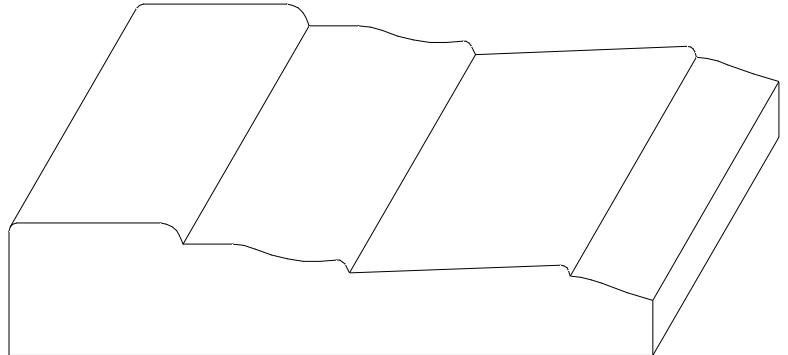
W-1084 21/32" x 3 3/16"
