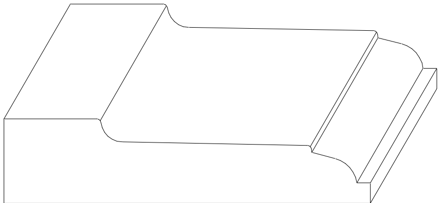
W-2275 3/4" x 3-7/16"
