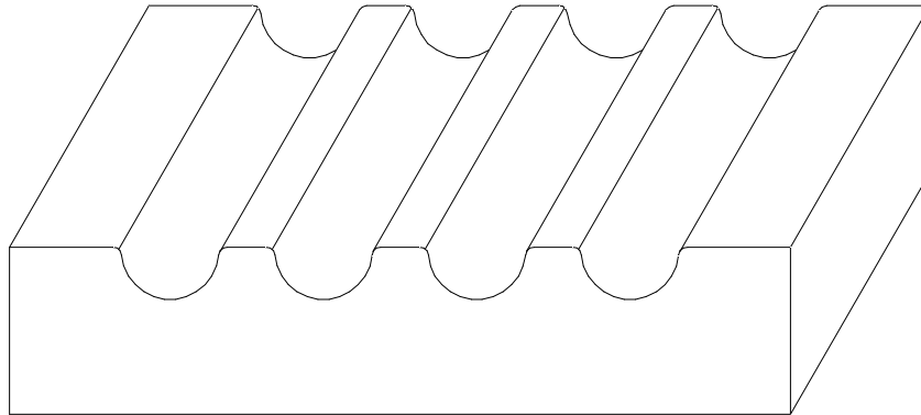
W-270 3/4" x 3 1/2"
