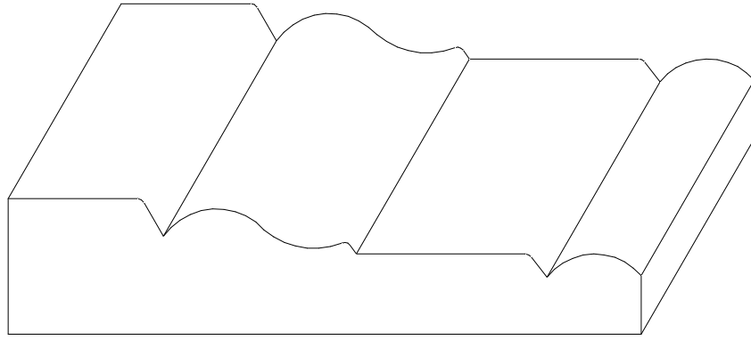
W-83 3/4" x 3 1/2"
