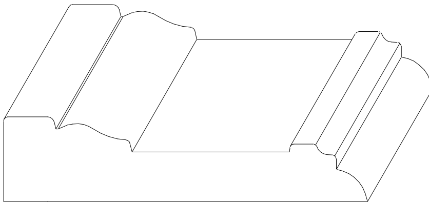
W-244 13/16" x 3 1/2"
