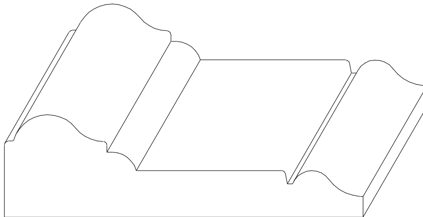
W-48 1" x 3 1/2"
