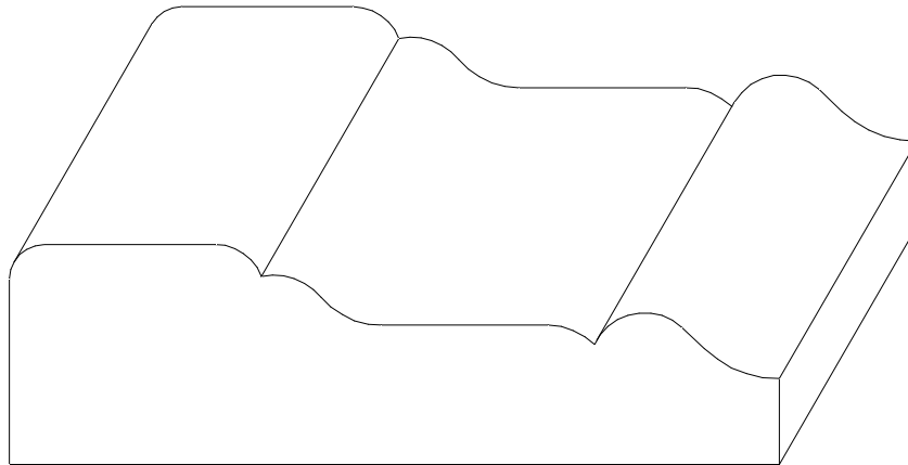
W-653 1" x 3 1/2"
