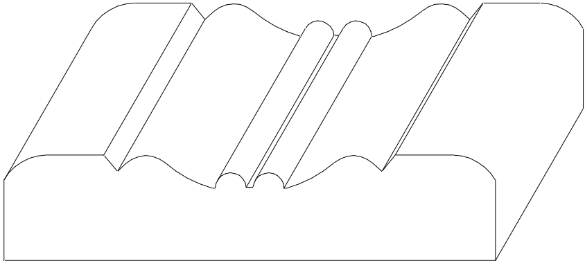
W-489 3/4" x 3 1/2"
