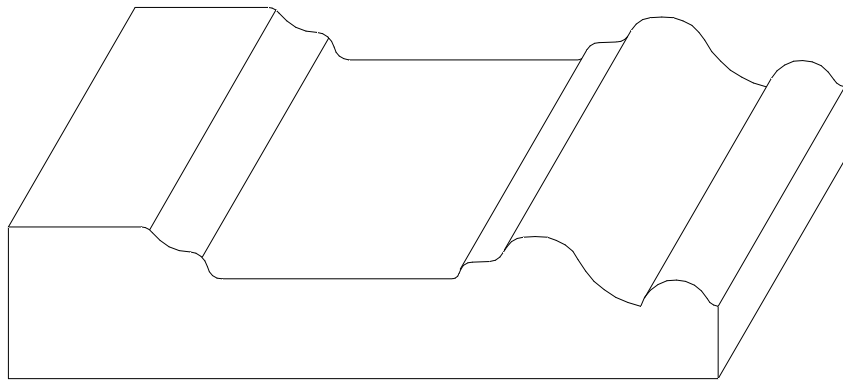
W-1034 3/4" x 3 1/2"
