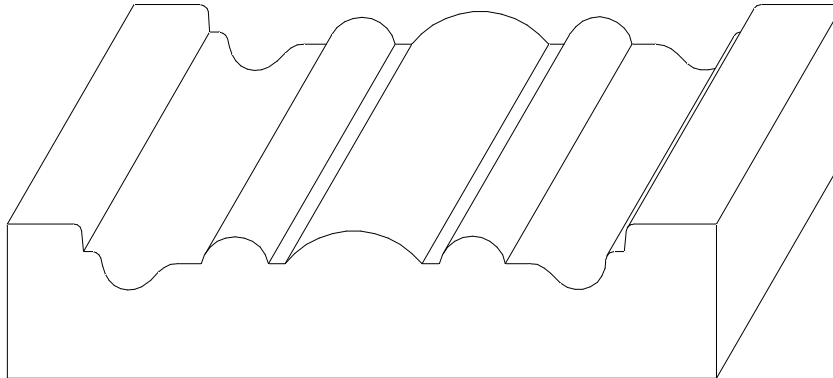
W-1596 3/4" x 3 1/2"
