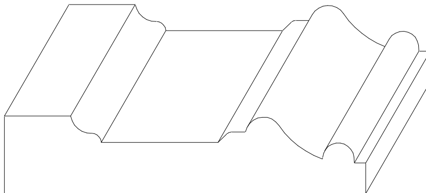
W-1638 3/4" x 3 1/2"
