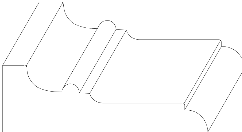
W-1634 1 3/16" x 3 1/2"
