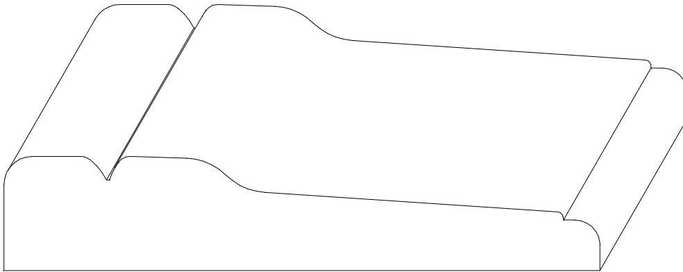
W-1597 13/16" x 4 1/4"
