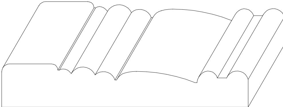
W-463 3/4" x 4 1/4"
