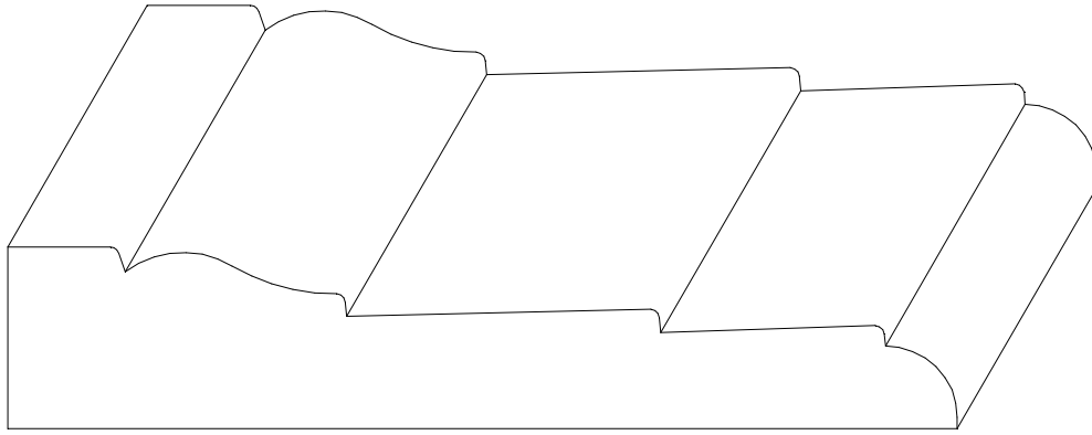
W-1512 13/16" x 4 1/4"
