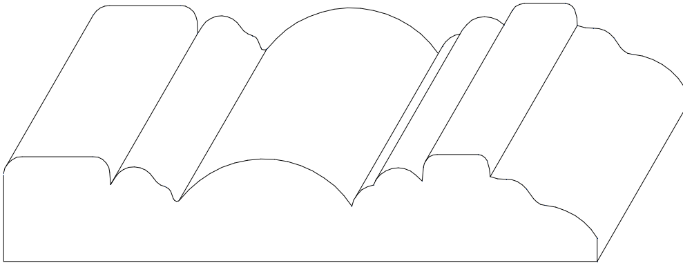
W-968 3/4" x 4 1/4"
