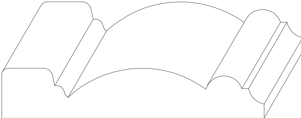
W-49 13/16" x 4 1/4"
