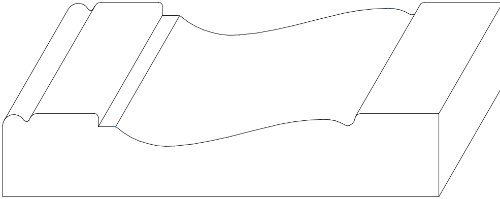
W-37 13/16" x 4 1/4"
