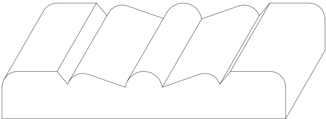
W-1331 3/4" x 4 1/2"
