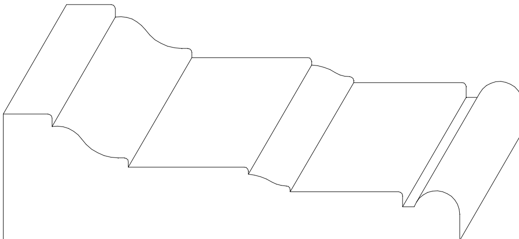
W-1189 1 1/4" x 4 1/2"
