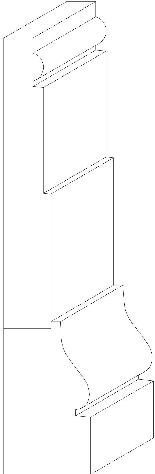
W-398AB 1 1/2" x 7 1/2"
