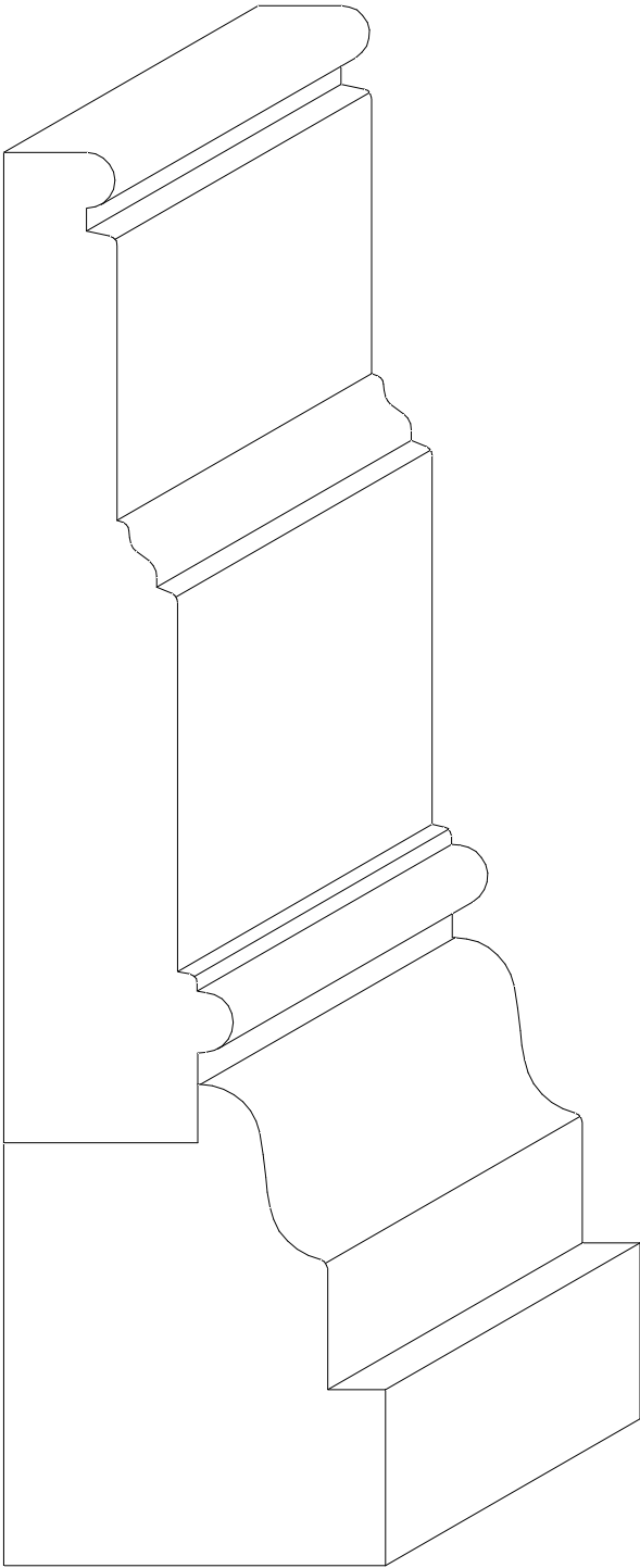
W-2155 1 5/8" x 6"
