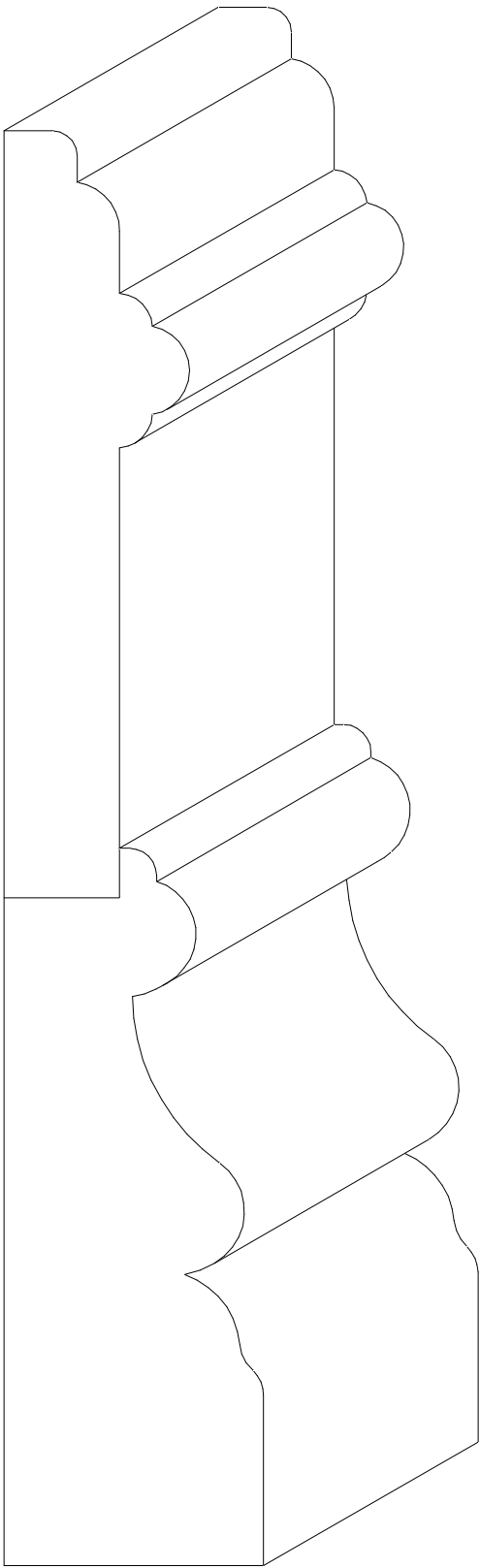
W-2094A&B 1 5/16" x 7 1/4"
