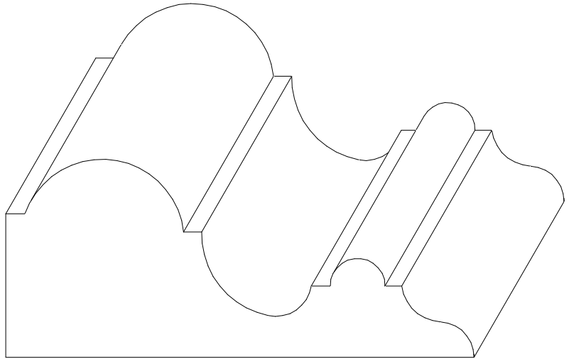
W-1545 1 3/8" x 3 1/4"
