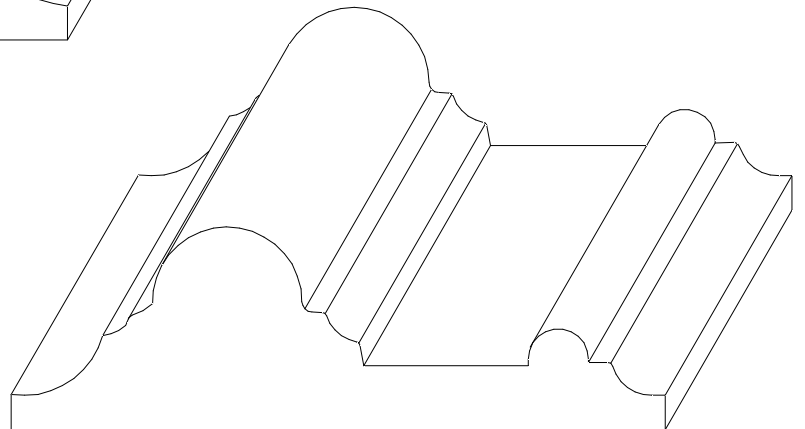
W-1352 1" x 3 1/4"
