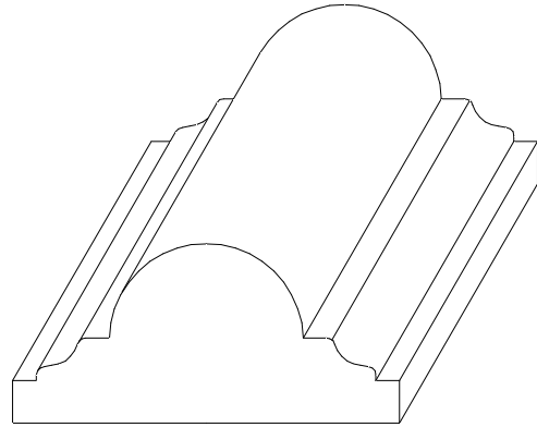
W-1032 13/16" x 1 3/4"
