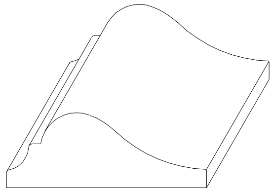
W-111 3/4" x 2"
