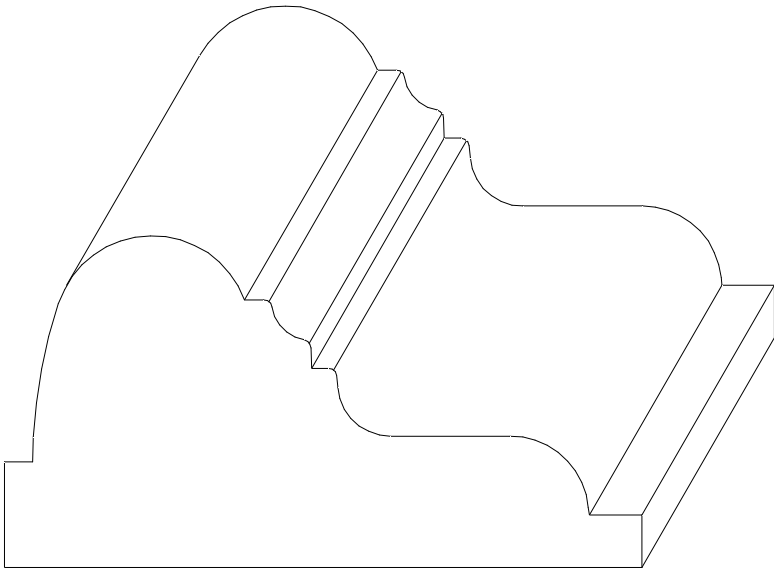
W-2184 1 9/16" x 3"
