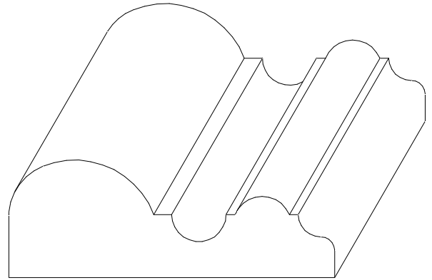
W-1297 13/16" x 2 1/4"
