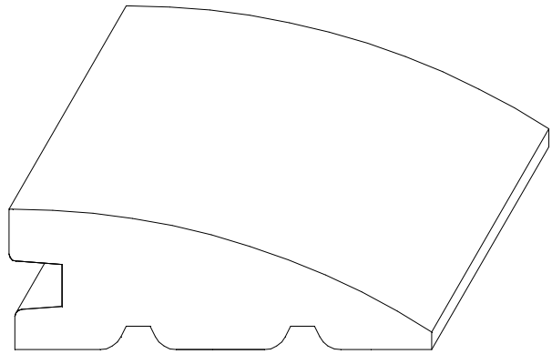
W-1864 3/4" x 2 1/4"
