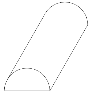
HALF ROUND 3/8" x 3/4"
