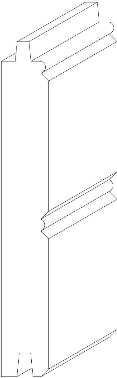
W-1052 3/4" x 5" FACE
