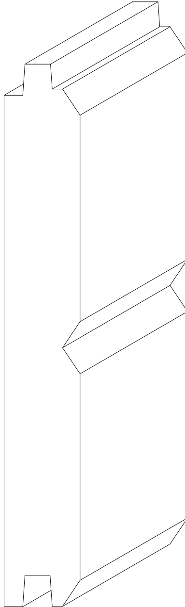
W-1844 3/4" x 5 3/16" FACE
