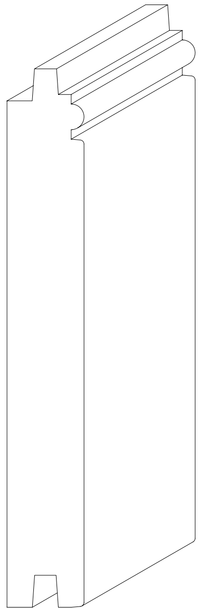
W-1774 3/4" x 5" FACE
