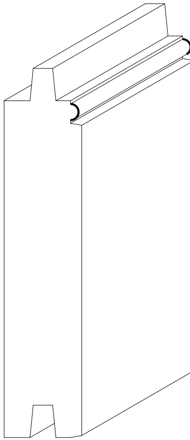
W-1366 3/4" x 3 1/4" FACE
