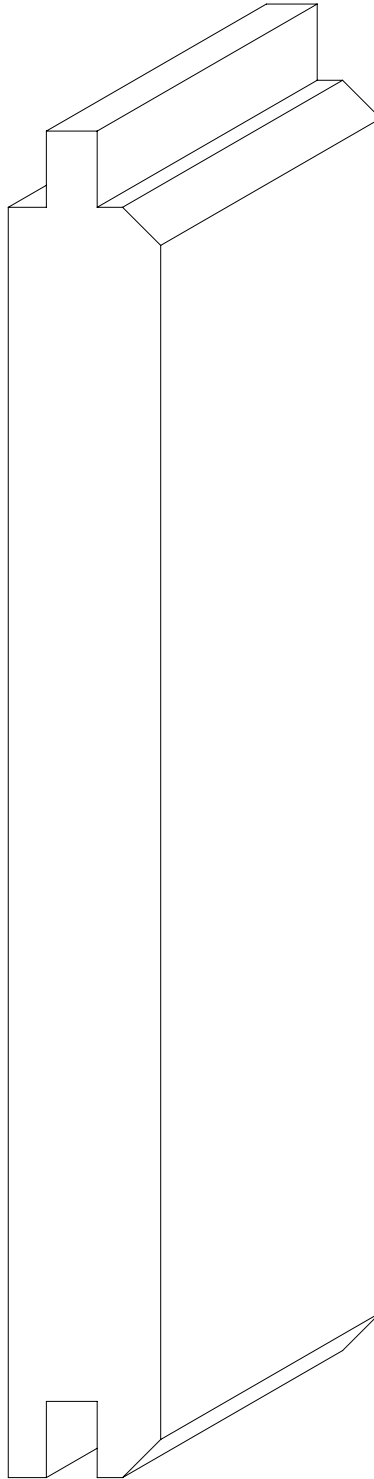
W-895 3/4" x 6 1/4" FACE
