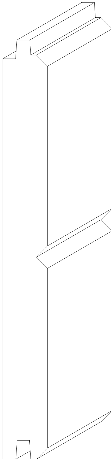
W-282 3/4" x 6 3/4" FACE
